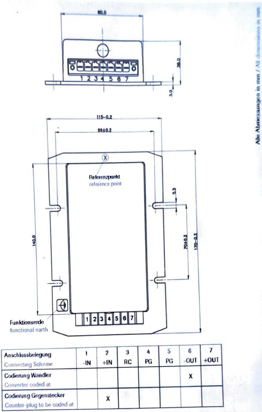
Physical dimensions of DC-DC converter
